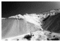
19 Canyon of Horim Creek near Sede Boqer in Negev Desert. The Middle East, May 10, 2000
