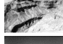
13 View of Bokek Creek canyon from the plateau, near Ein Bokek. The Middle East, May 20, 2000
