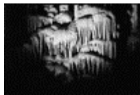
18 Yellow tainted stalactites in Sorek Cave, west from Jerusalem. The Middle East, December 30, 2000
