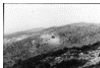
20 Shimshon Cave at Sorek River, west from Jerusalem. The Middle East, December 30, 2000
