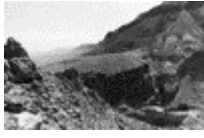
10 View of the canyon and Dead Sea from Maal Bokek trail. The Middle East, March 25, 2000
