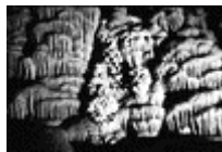
16 Wall of stalactites in Sorek Cave, west from Jerusalem. The Middle East, December 30, 2000
