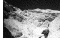
18 Canyon of Horim Creek near Sede Boqer in Negev Desert. The Middle East, May 10, 2000
