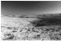
08 Hills in Negev Desert 2 miles north from Beer-Sheva. The Middle East, December 16, 2000
