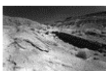
03 Multicolor sands in Big Crater (Makhtesh Gadol) in Negev Desert. The Middle East, March 11, 2000
