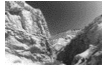
17 Canyon of Horim Creek near Sede Boqer in Negev Desert. The Middle East, May 10, 2000
