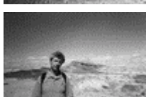
09 A.S. in Big Crater (Makhtesh Gadol) in Negev Desert. The Middle East, March 11, 2000
