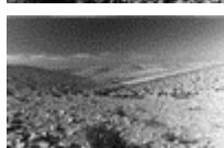
19 Negev Desert on hills opposite to Golda Meir Park. The Middle East, March 11, 2000
