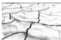
36 After rain in Negev Desert 1 mile north from Beer-Sheva. The Middle East, November 11, 2000
