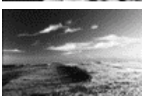
34 Hills with planted pines in Negev Desert, 1.5 miles north from Beer-Sheva. The Middle East, December 16, 2000
