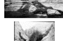
37 New road through chalkstone of Negev Desert 1 mile north from Beer-Sheva. The Middle East, November 11, 2000
